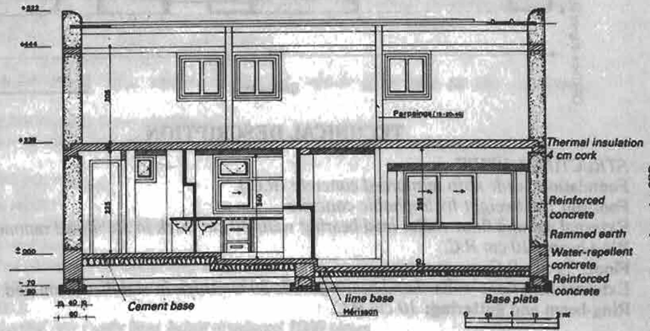
FIGURE 113: LONGITUDINAL SECTION
