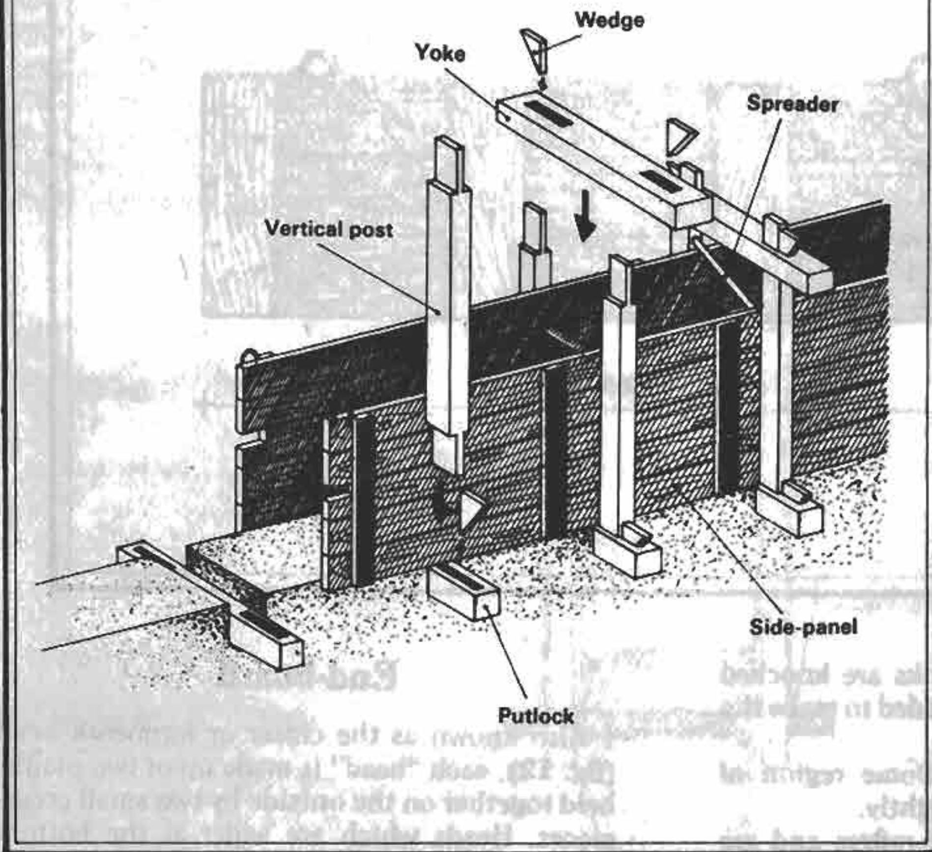
FIGURE 11: SHUTTERING FROM THE AUVERGNE REGION, FRANCE.
