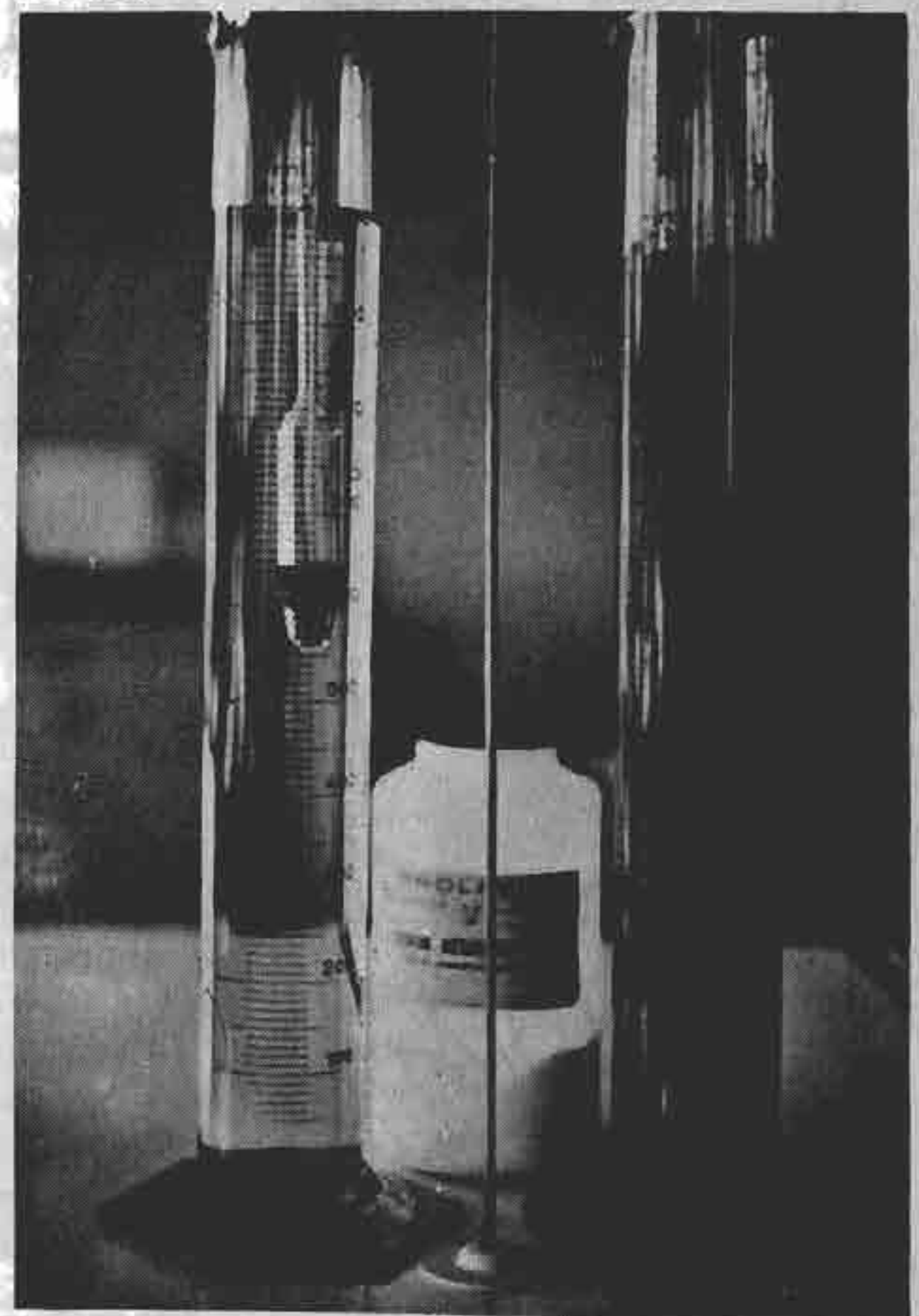
FIGURE 248: EQUIPMENT FOR SEDIMENTATION TEST (1) BORE-SHAPED DENSIMETRE GRADUATED FROM 995 TO 1030, 2 1 LITRE CYLINDERS, 1 THERMOMETER, 1 PLUNGER, SEPERATING AGENT, 1 RECORD SHEET, 1 WATCH).
