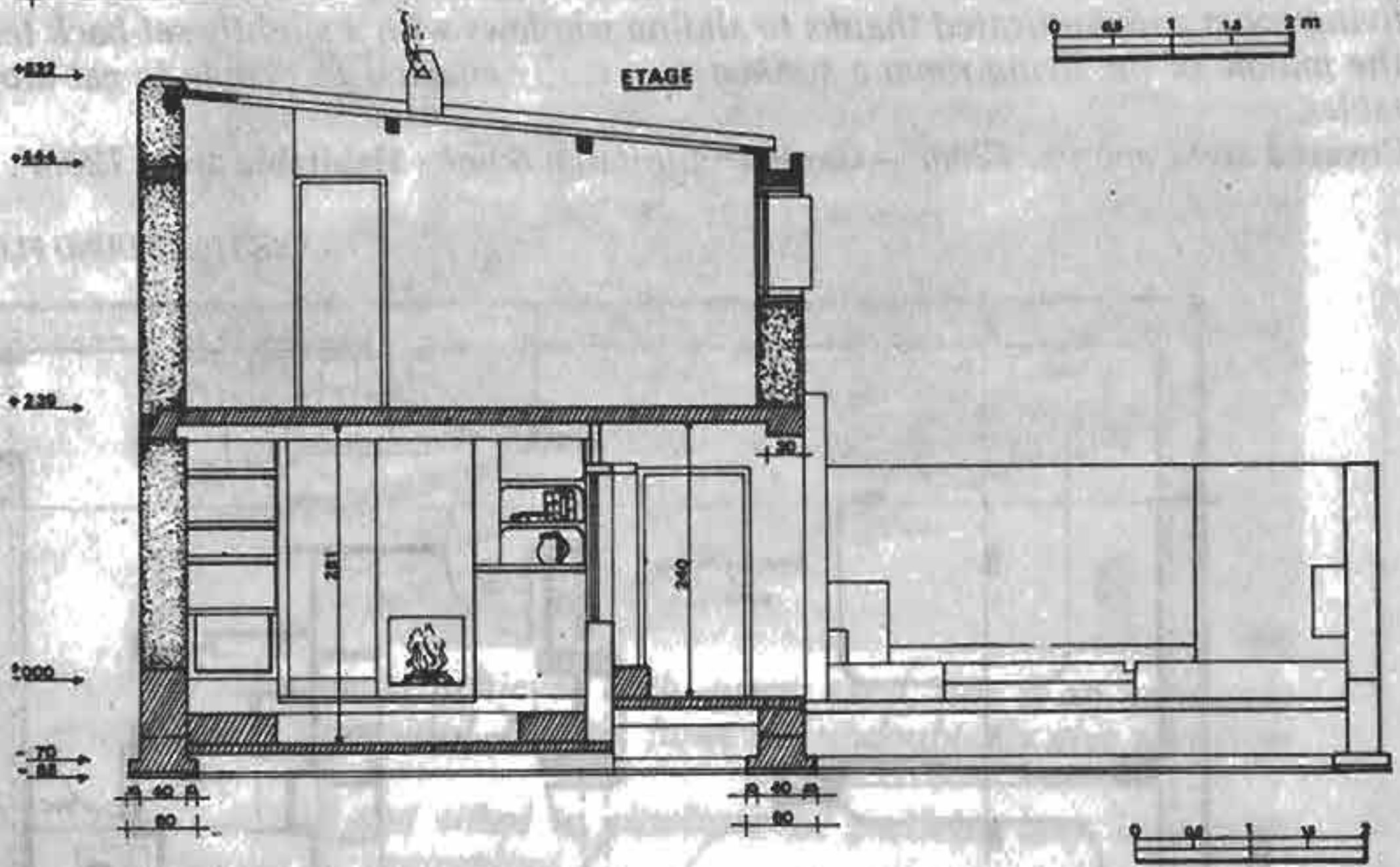
FIGURE 112: TRANSVERSE SECTION
