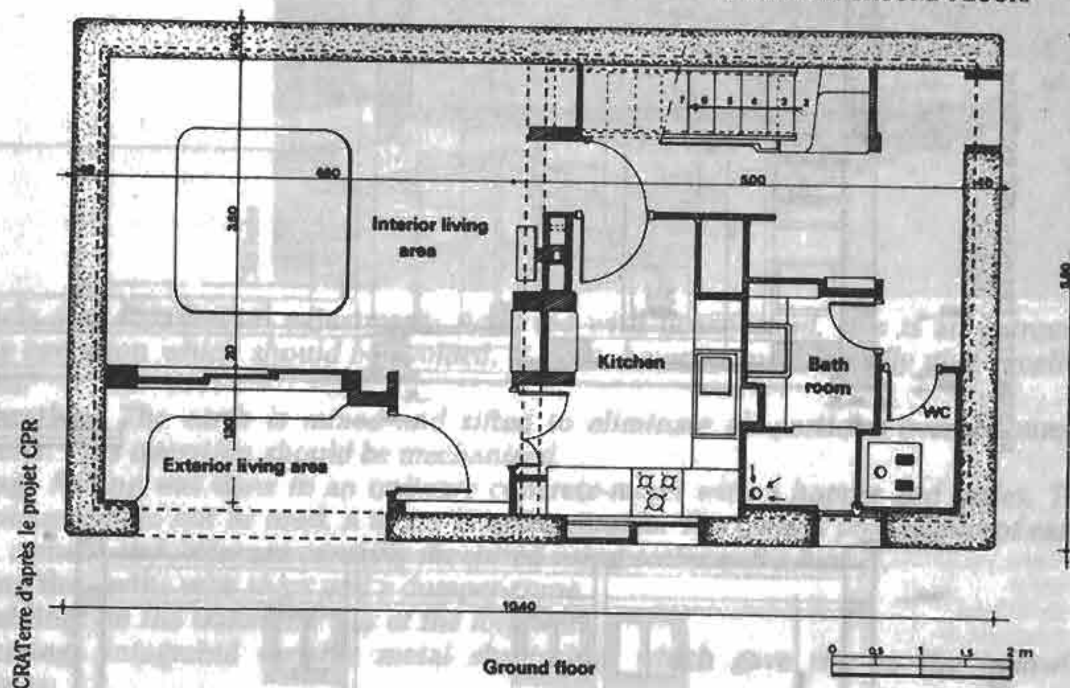
FIGURE 110: GROUND FLOOR.
