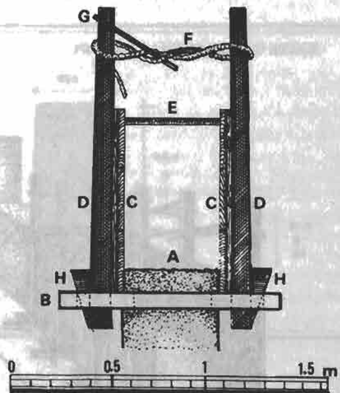
FIGURE 8: FORMWORK FROM THE LYONNAIS REGION (FRANCE).
