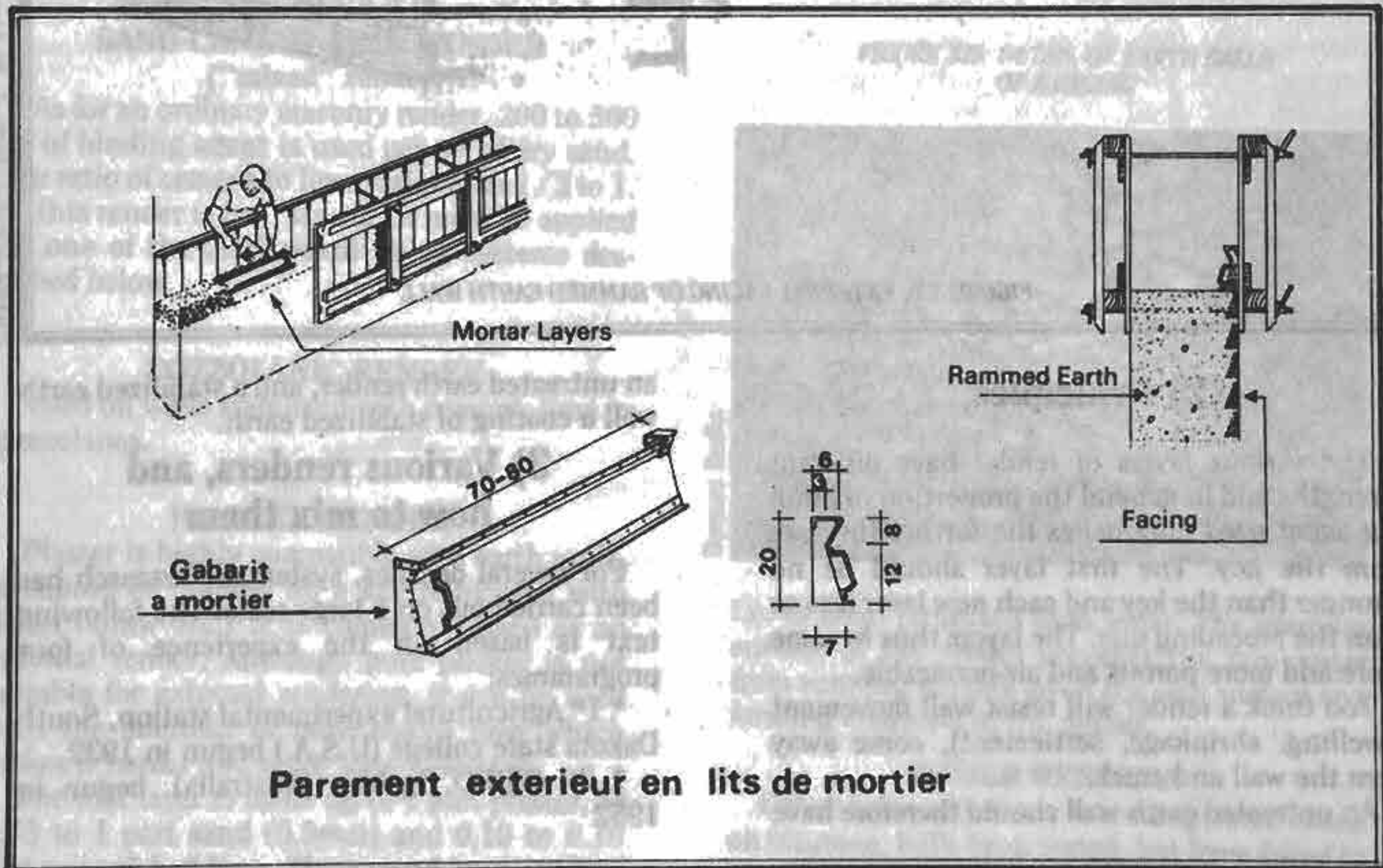
FIGURE 325: EXTERNAL FACING OF MORTAR LAYERS
