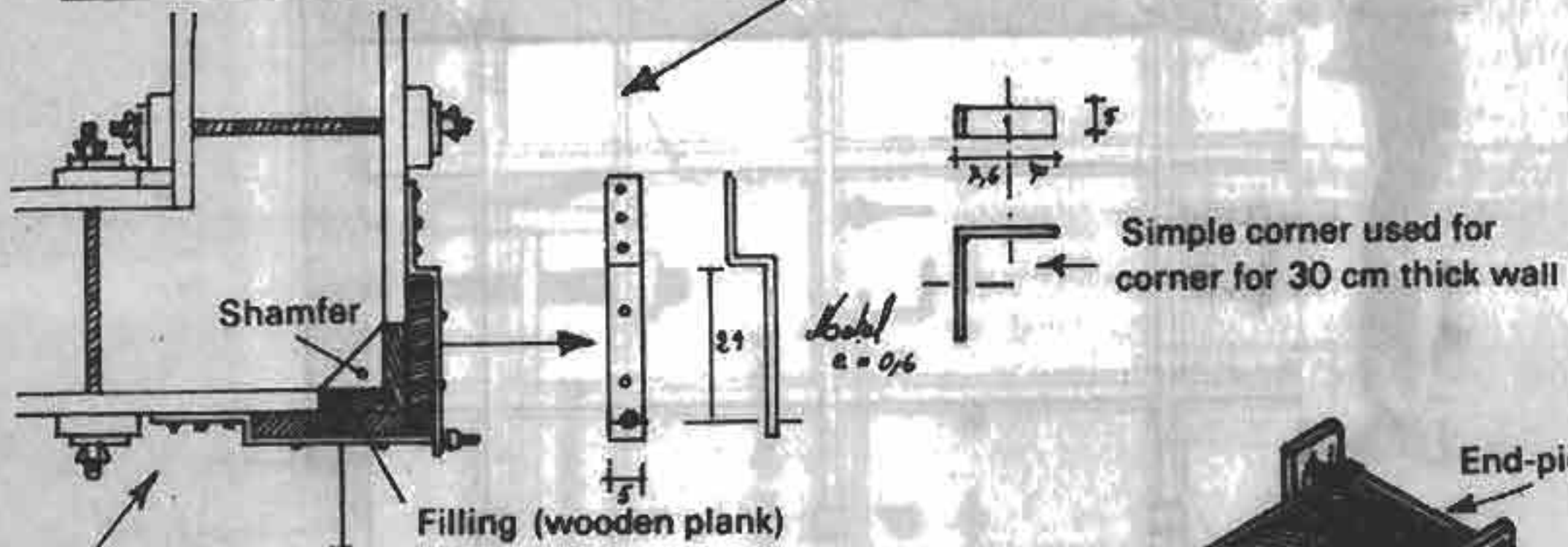
Detail of corner
