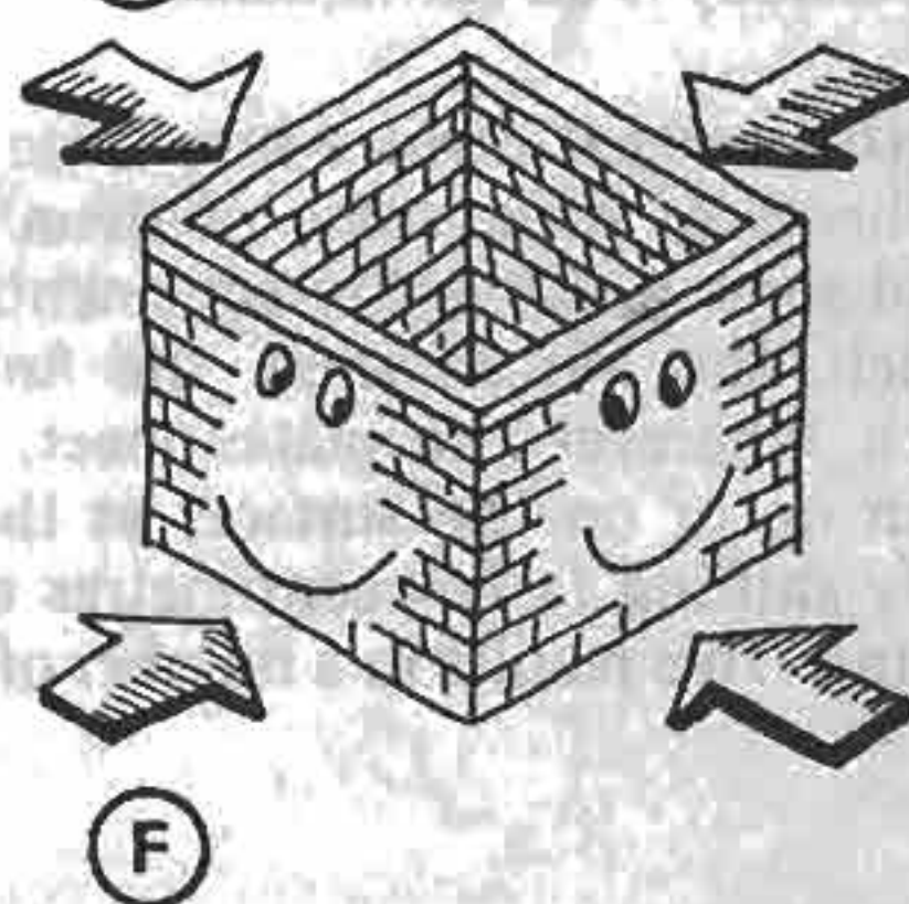
D - A RING-BEAM WILL IMPROVE RESISTANCE FURTHER. E - TWO PARALLEL WALLS (WITHOUT BRACING) WILL COLLAPSE IF SUBJECTED TO TRANSVERSE PRESSURE. F - A "BOX" FORMED BY RIGHT-ANGLED RING-BEAMS WILL HAVE GREATER RESISTANCE.
