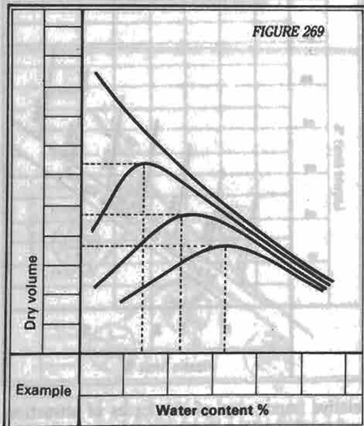
Compaction stresses
