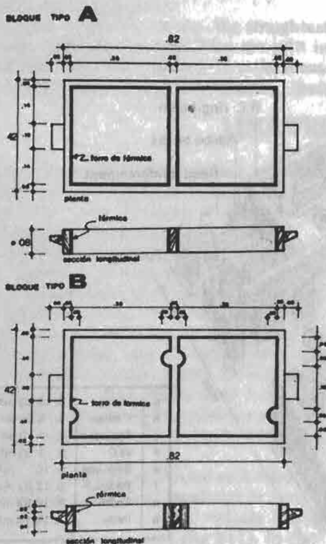
FIGURE 203: MOULDS USED AT CAYALTI.
