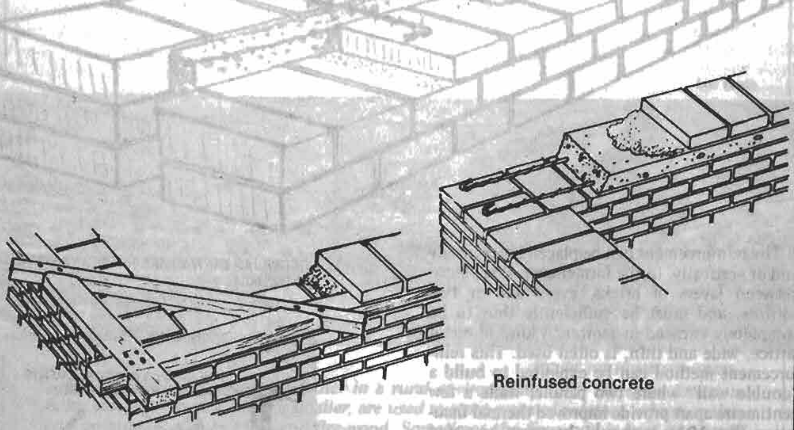
FIGURE 190: VARIOUS TYPES OF RING-BEAM
