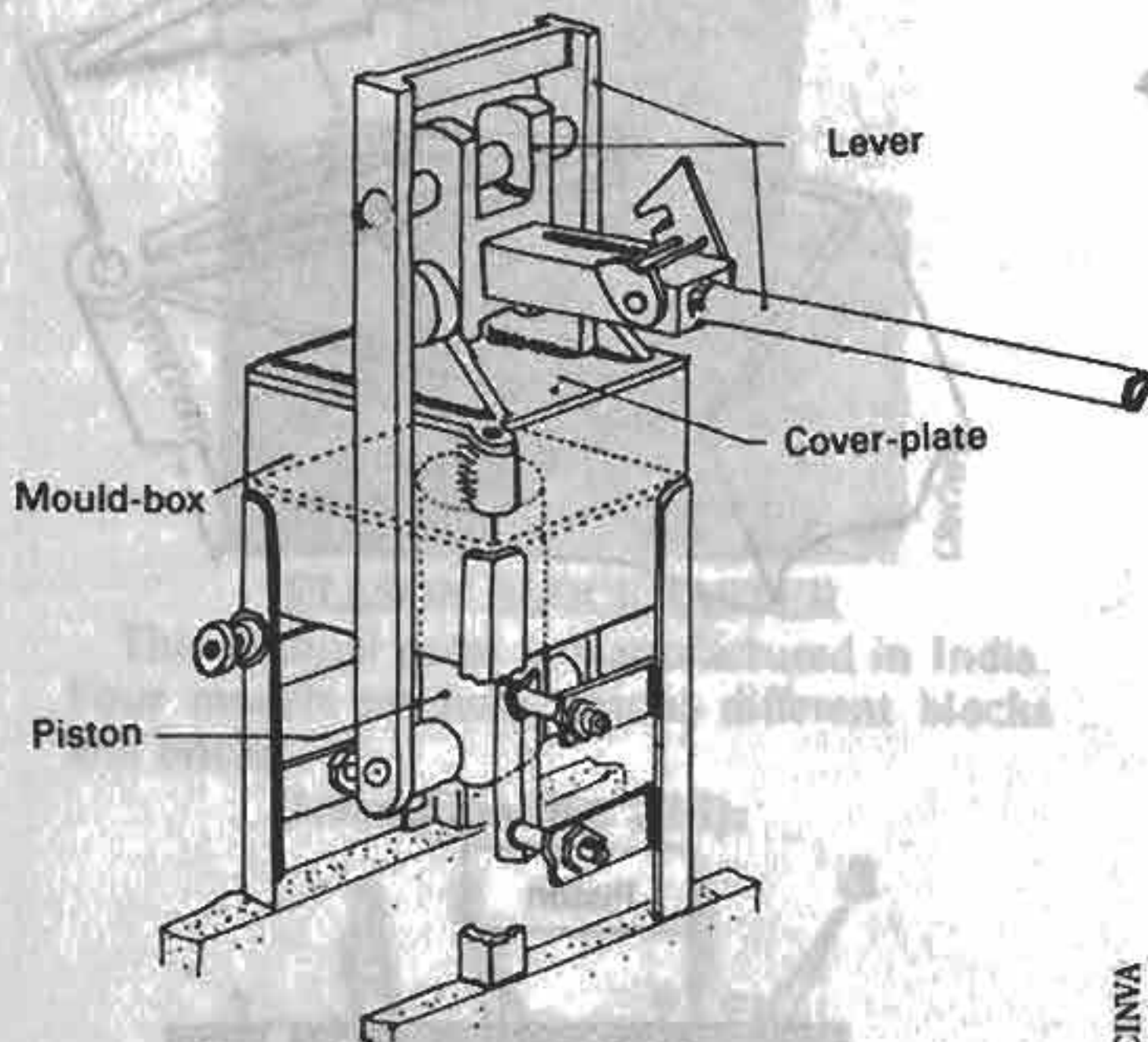
FIGURE 219: CINVA-RAM PRESS
