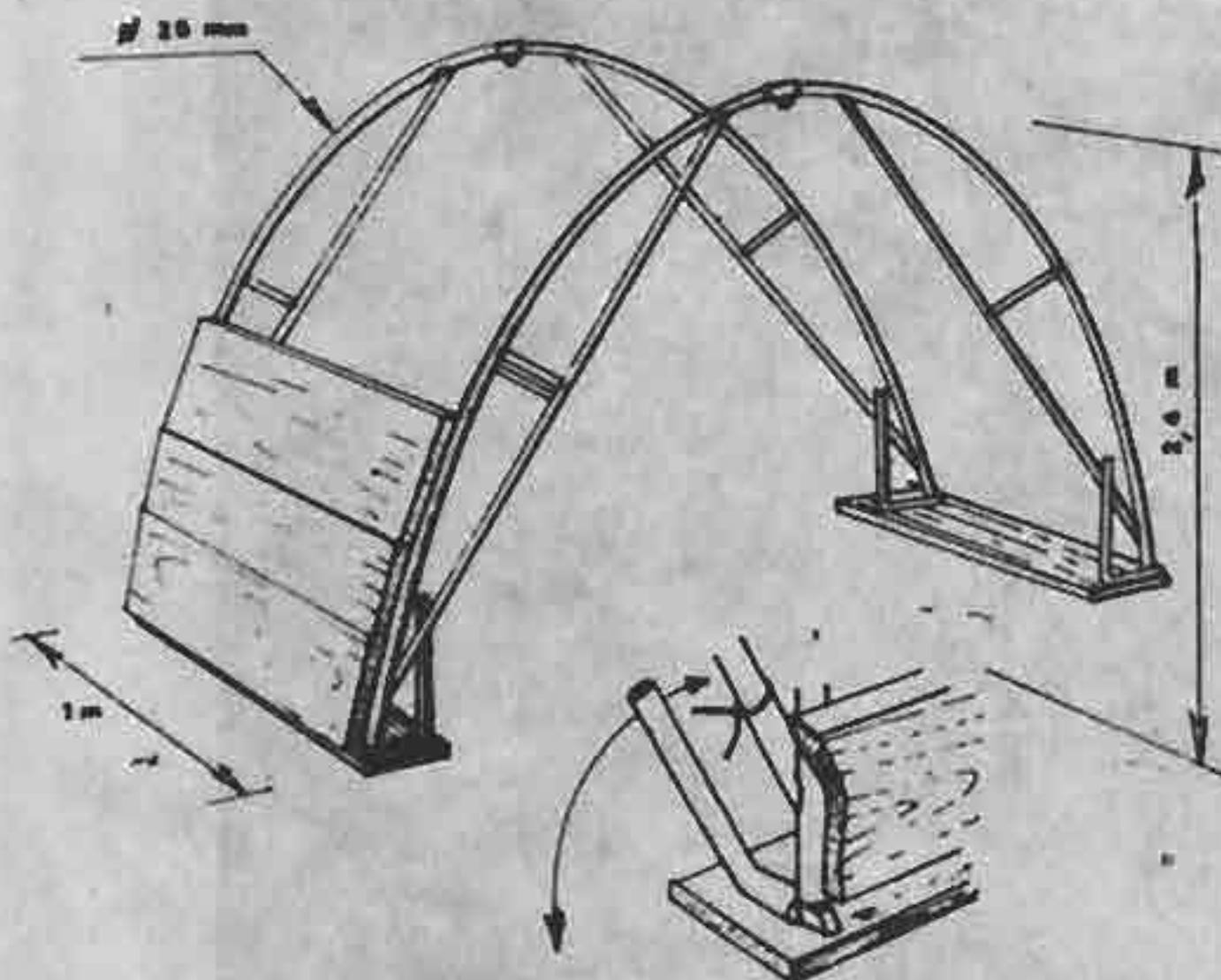
FIGURE 306: EXPERIMENTAL SHUTTERING WITH CAM TO FACILITATE REMOVAL
