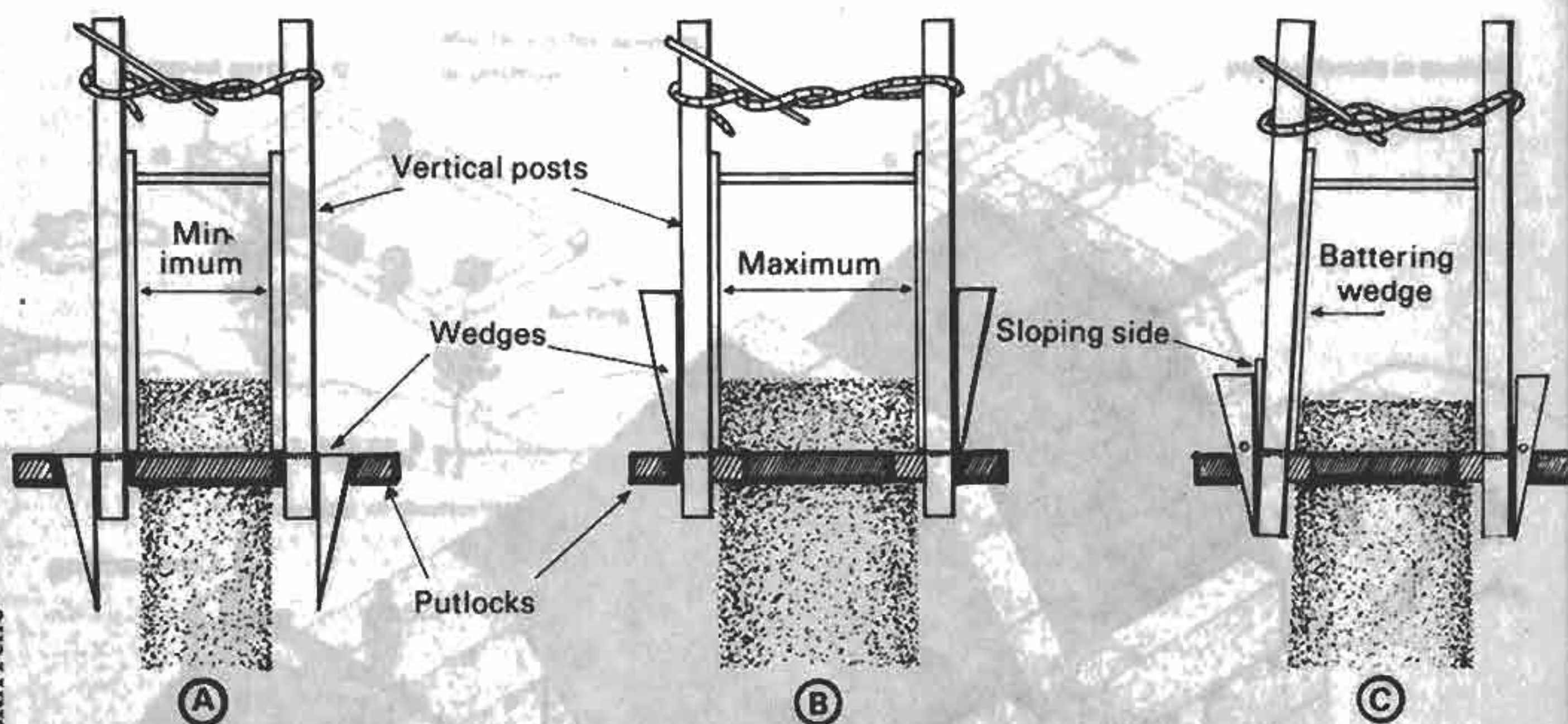
FIGURE 14 (a) and (b): THE GAP BETWEEN THE SIDE-PANELS VARIES ACCORDING TO THE DEPTH TO WHICH THE WEDGES ARE DRIVEN IN — (c) HOW TO ACHIEVE A BATTERED WELL.
