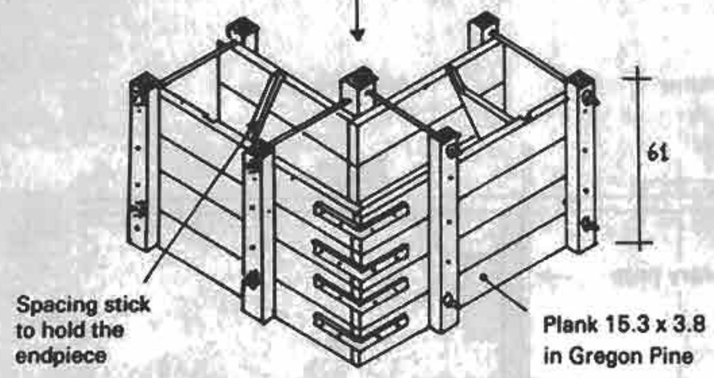
Corner shuttering
