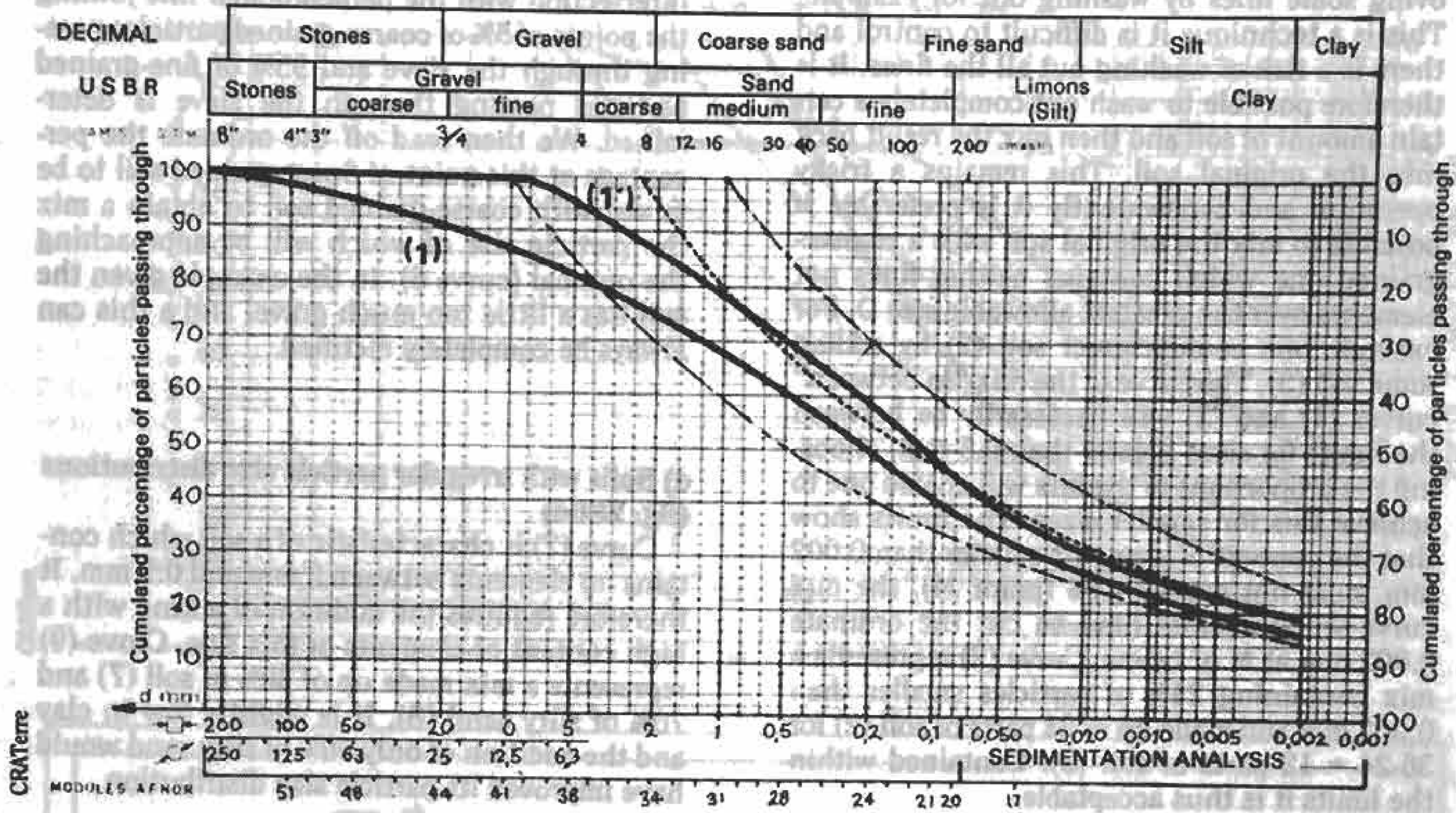
FIGURE 280a: FINDING THE PROPORTIONS OF THE MIX REQUIRED TO ATTEMPT TO ACHIEVE, FROM THE STARTING-POINT OF DIFFERENT SOILS, A SOIL FALLING WITHIN THE LIMITS APPROPRIATE FOR RAMMED EARTH. - CONTINUOUS LINES: THE TWO ORIGINAL SOILS - LIGHT BROKEN LINES: THE LIMITS APPROPRIATE FOR RAMMED EARTH AND THE IDEAL CURVE - BOLD DOTTED/BROKEN LINES: THE MIXED SOIL CURVE
