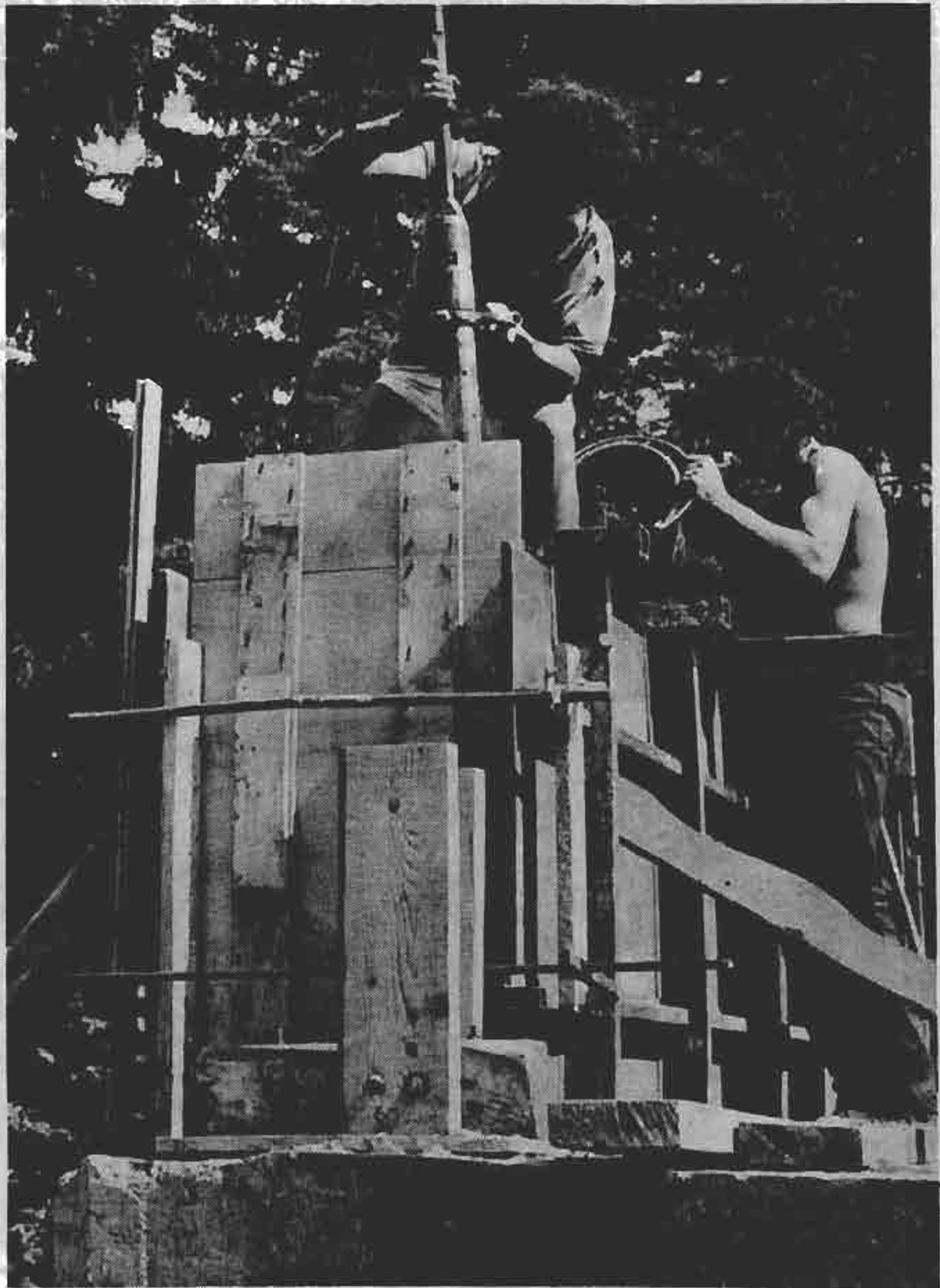
▲ FIGURE: 96 EXPERIENCE AT LE PIN (ISERE, 1975) OF THE "PALAFITTE" TEAM, PART OF THE SCHOOL OF ARCHITECTURE OF GRENOBLE - CIRCULAR RAMMED EARTH BUILDING.
