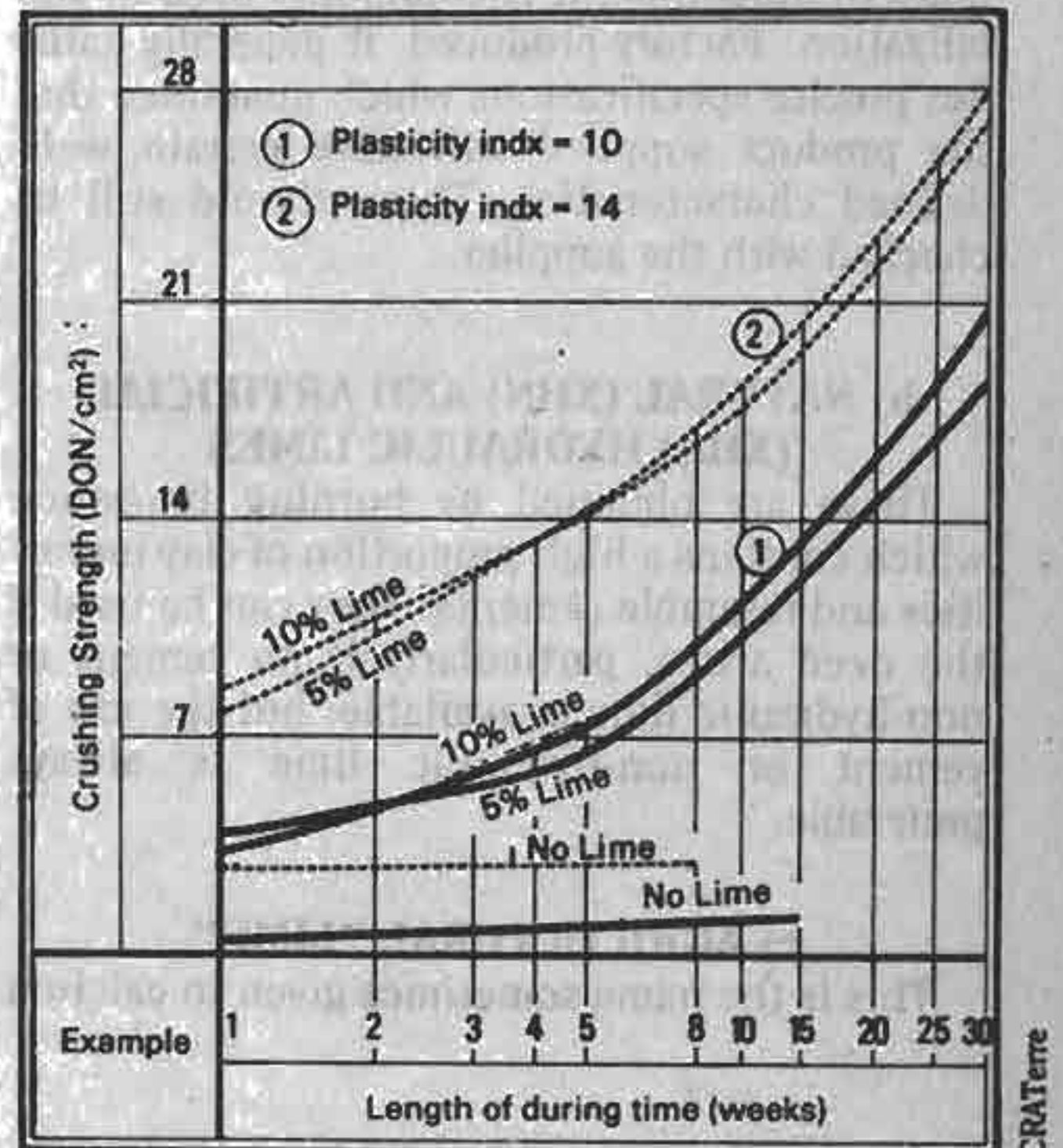
FIGURE 288: LENGTH OF CURING TIME AND STRENGTH
