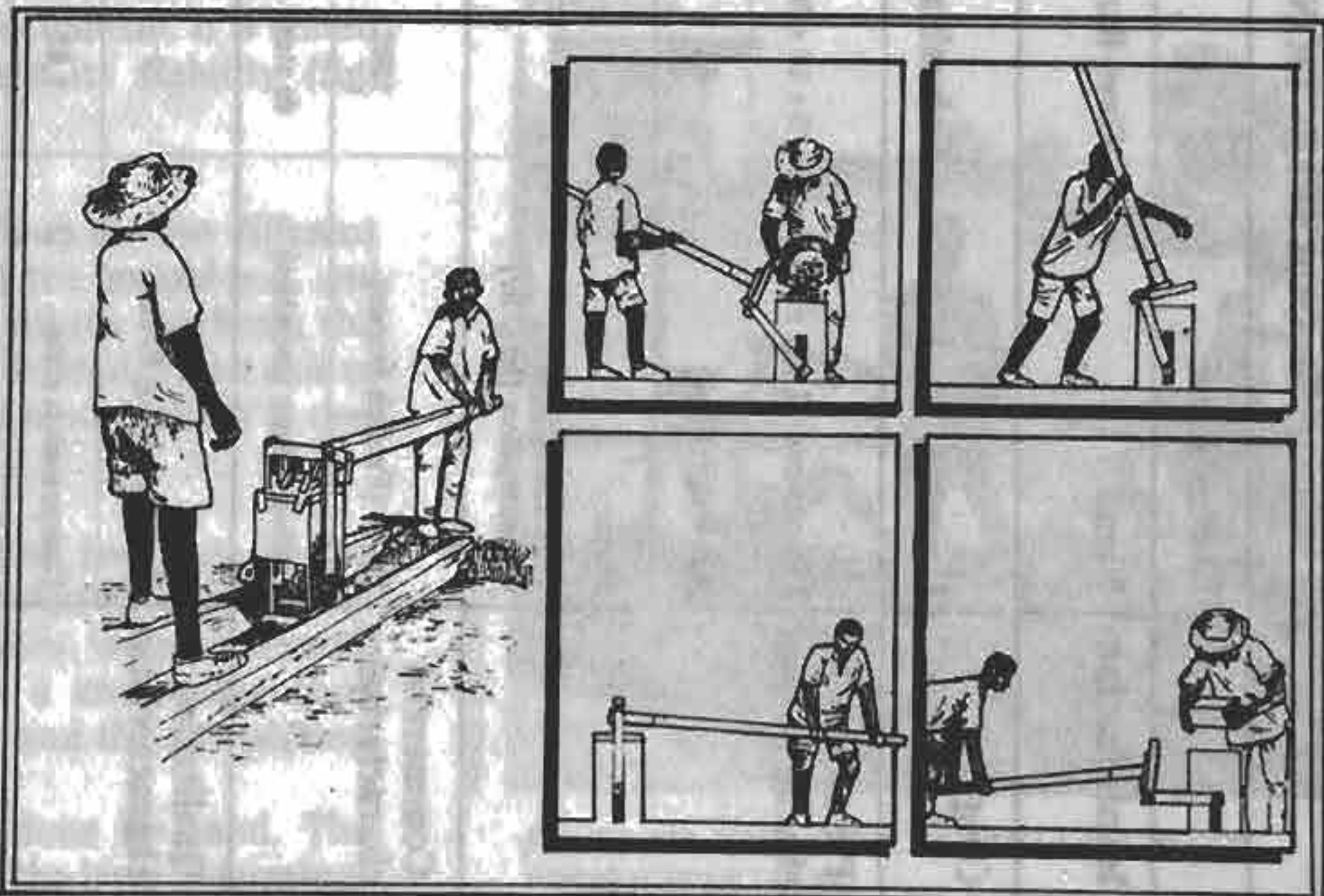
FIGURE 222: TEK-BLOCK PRESS — FILLING THE MOULD — COMPACTING — REMOVING THE BRICK
