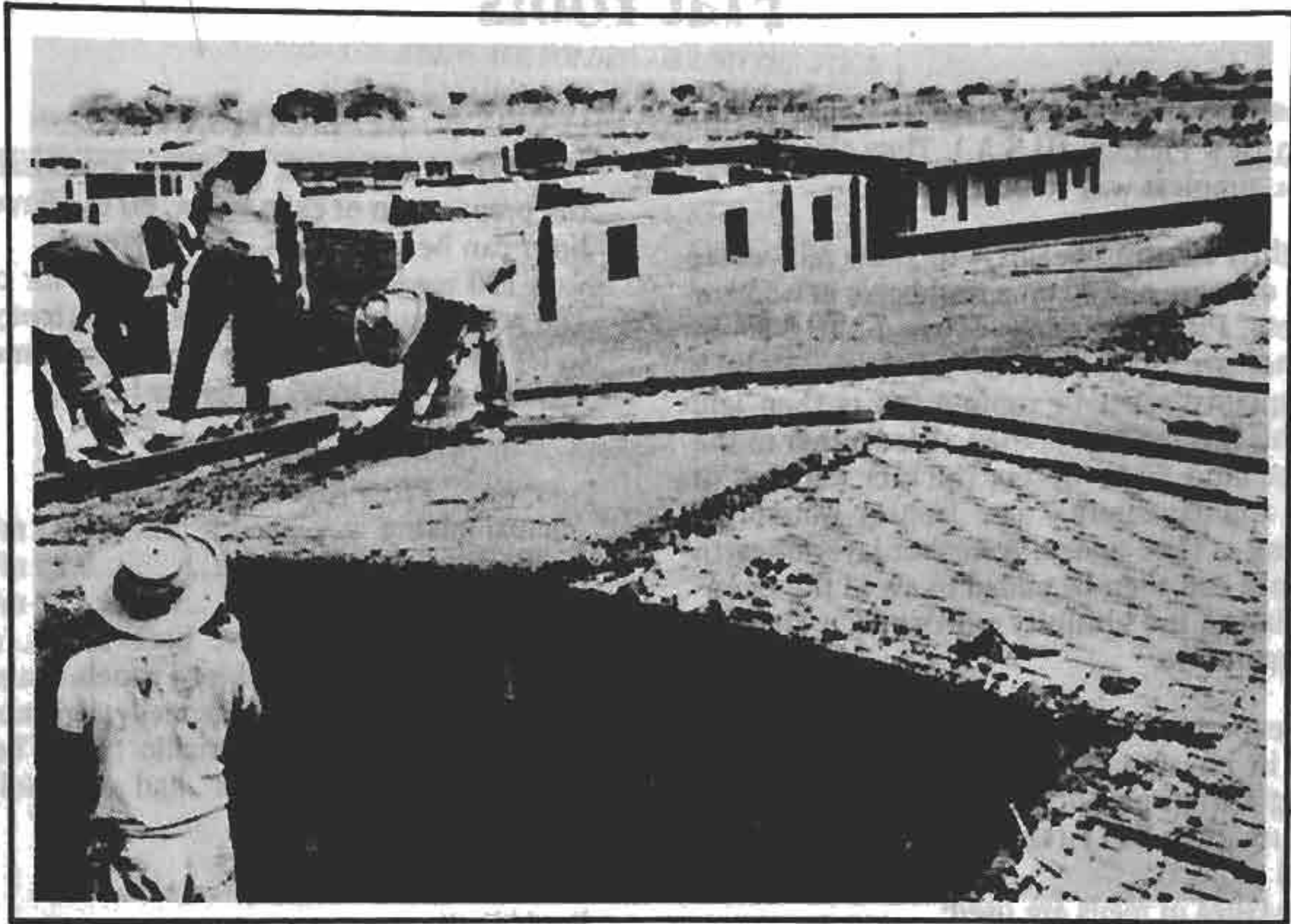
FIGURE 301: POURING STABILIZED EARTH ONTO THE ROOF OF ONE OF THE CAYALTI HOUSES (PERU); CF. CHAPTER ON "ABODE".
