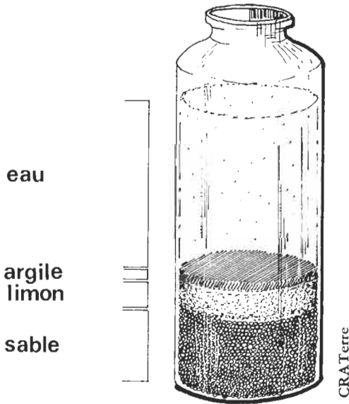
FIGURE 260 : SEDIMENT SIMPLIFIE
