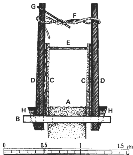
FIGURE 8 : BANCHE LYONNAISE
