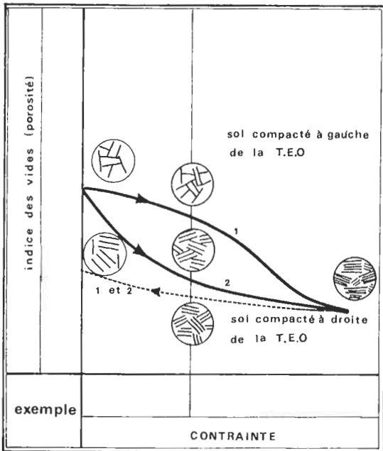
FIGURE 277 : COMPRESSION - DECOMPRESSION
